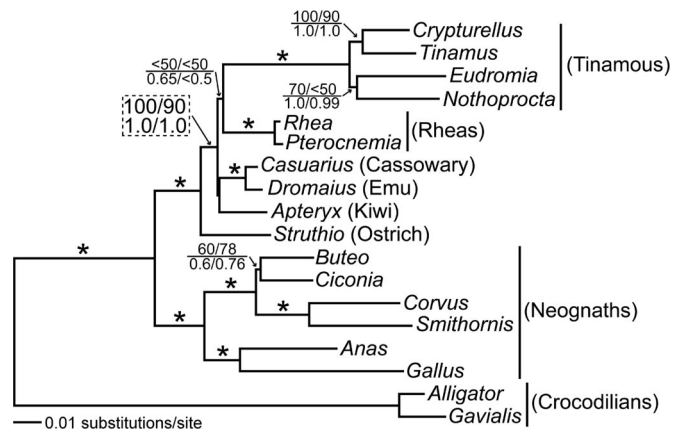
Fig. 2. Phylogenetic analyses including crocodylian outgroups and two passerine birds ( Corvus and Smithornis ) strongly support the conventional position of the avian root and ratite polyphyly. Analyses were conducted by using all sequences that could be aligned between crocodylians and birds (4,668 bp). Support measures are unpartitioned ML bootstrap (Upper Left), MP bootstrap (Upper Right), unpartitioned Bayesian posterior probability (Lower Left), and partitioned Bayesian posterior probability (Lower Right). Branch lengths shown reflect the unpartitioned ML analysis. Branches for which all support measures were 100% or 1.0 are indicated with an asterisk; the branch with no support values had <50\% bootstrap support and <0.5 Bayesian posterior probability in all analyses. MP and ML analyses conducted after Y coding produced similar results (not shown).
